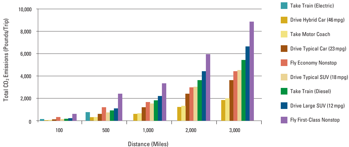
Figure 25. Comparing Carbon Footprints across All Modes: Family of Four
