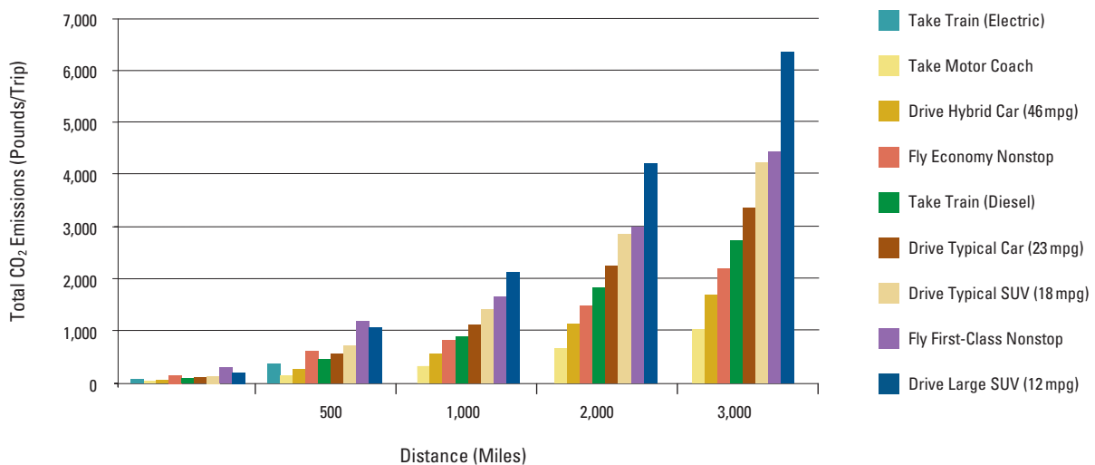
Figure 24. Comparing Carbon Footprints across All Modes: Two Travelers
