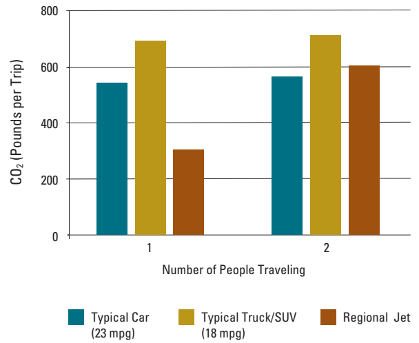
Figure 9. Total CO 2 Emissions, 500-Mile Trip
